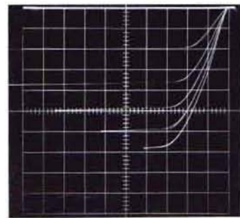
Collector current vs collector voltage. Vertical deflection is 10 A/div, horizontal deflection is 1.0 V/div. Base drive is 500 mA/step (top curve is 2.5 A).
