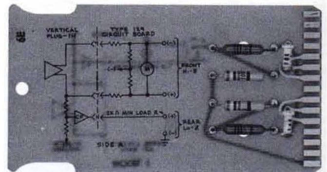
PASSIVE DIVIDER CIRCUIT CARD Order 018-0002-00
