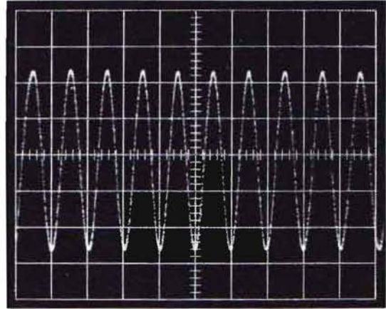
Horiz: 0.2 ns/cm; Vert: 100 mV/cm External trigger, UHF Sync Mode
