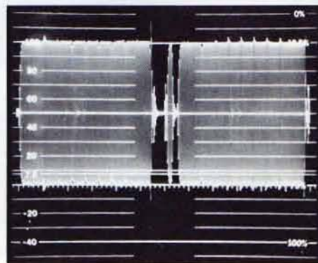
Fig 3. Modulated stairstep signal. 2 H SWEEP, DIFF GAIN response.
