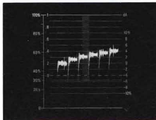
Fig. 2—Differential Gain presentation using a modulated staircase signal. The right side of the graticule is marked in % of gain distortion. From white to black luminance levels the indicated gain distortion is 4%.
