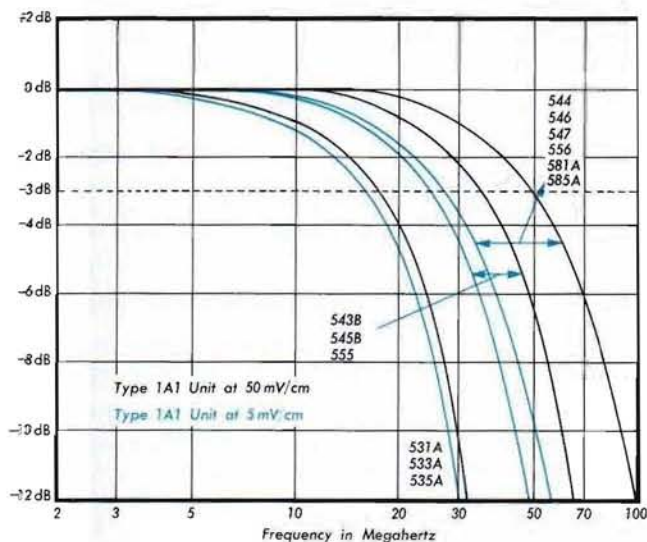
TYPICAL BANDWIDTH
