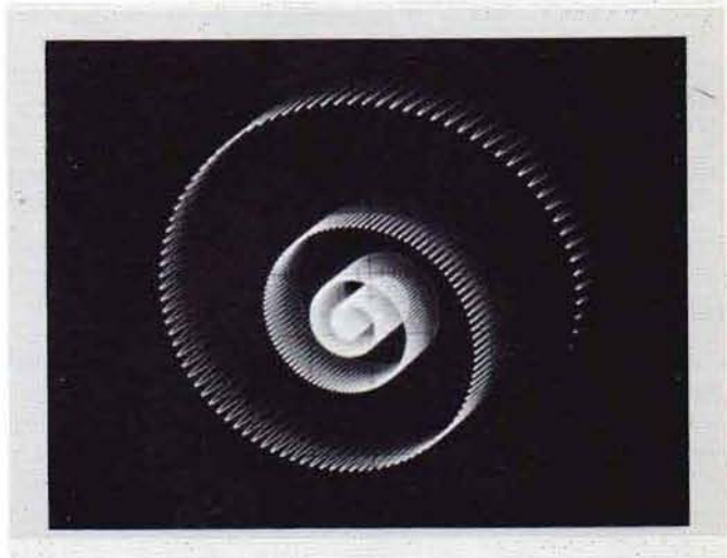
Displayed is a low-frequency damped sine wave with 90^\circ phase difference between X and Y inputs. A 1-MHz timing sine wave is also applied to the X, Y and Z input. Intensity modulation with the 1-MHz timing waveform adds the third display parameter and creates the illusion of depth.
