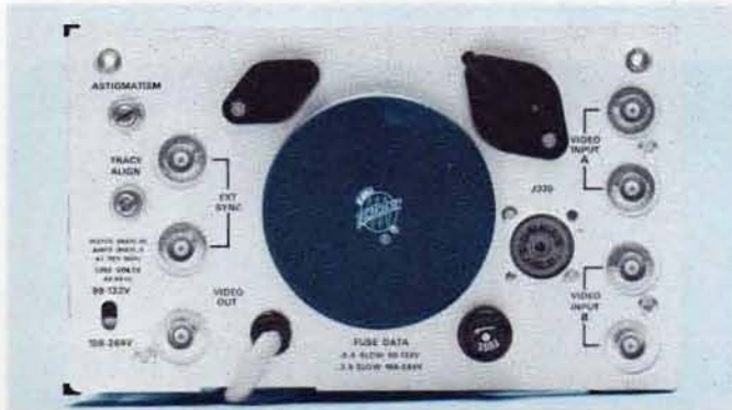
Rear panel of Type 528 Waveform Monitor.
