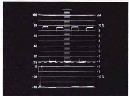
Line sweep presentations of the luminance (Fig. 4), Red (Fig. 5), Green (Fig. 6), and Blue (Fig. 7), components of the NTSC color bar signal.
