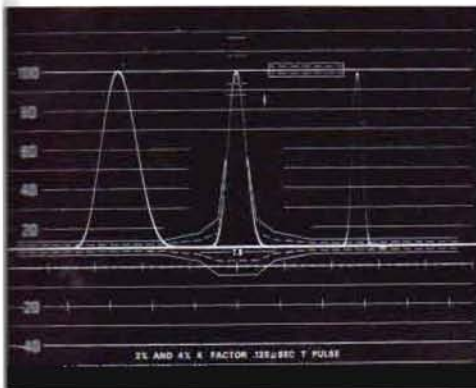
Multiple exposure. Left: 2T. Center: T. Right: \frac{1}{2} T Sine 2 , 0.25, 0.125, 0.0625 \mu s HAD.
