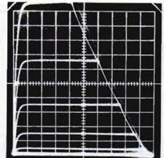
NPN TRANSISTOR
