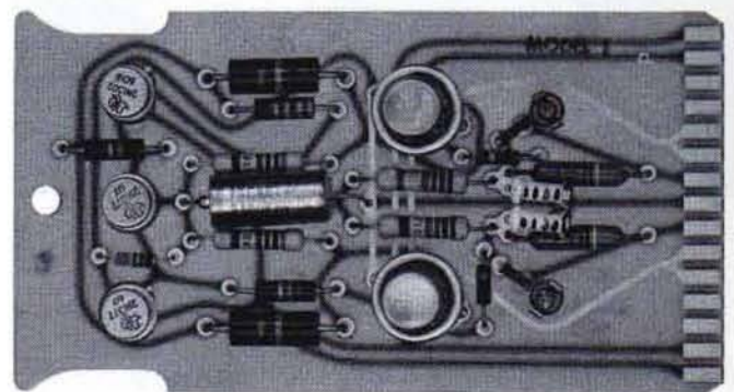
CATHODE-FOLLOWER CIRCUIT CARD Order 018-0001-00
